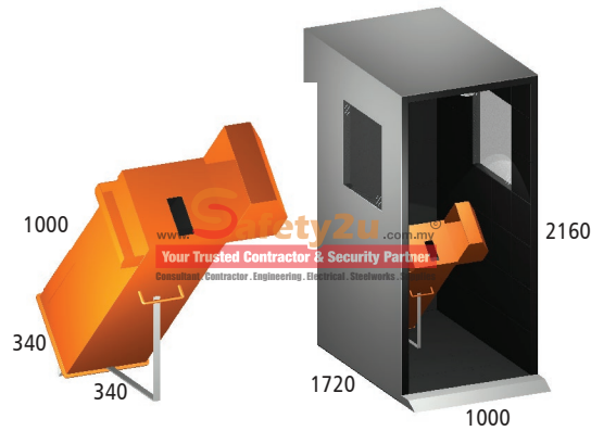
S2U CLEARING CHAMBER & BOOTH
